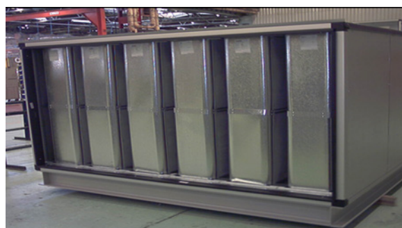
Fig 38: Sound Attenuator
