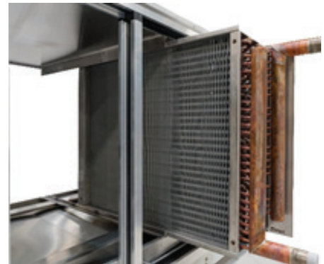
Fig 21: Coils Mounted on Slide Rail for Easy removal
