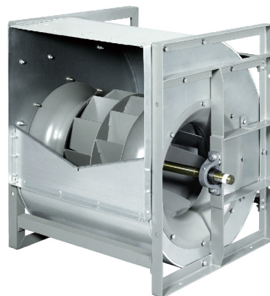
Fig 25: Backward Curved Fan
